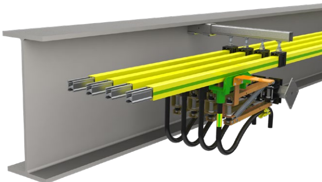
Horizontal installation of conductor rails / insertion of Current Collectors from below
