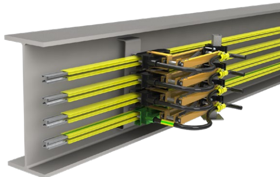
Lateral installation of conductor rails / insertion of Current Collectors from the side
